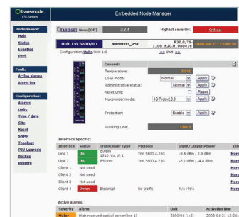
Fig. 3 The Element Node Management interface
