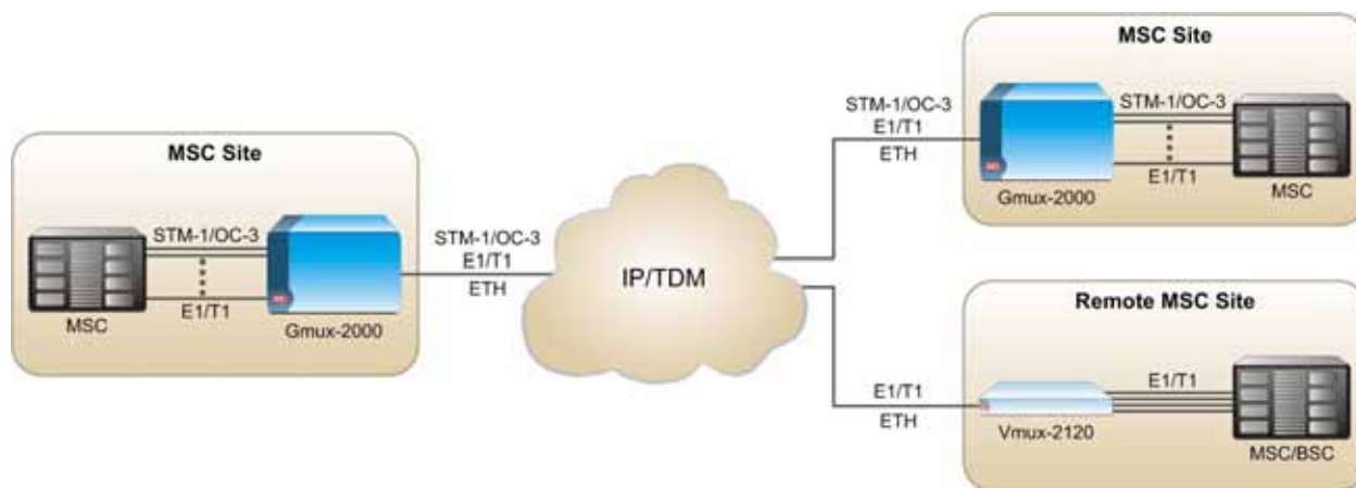
Figure 2. VCA-E1/VCA-T1 in an Inter-MSC Application for Cellular Operator
