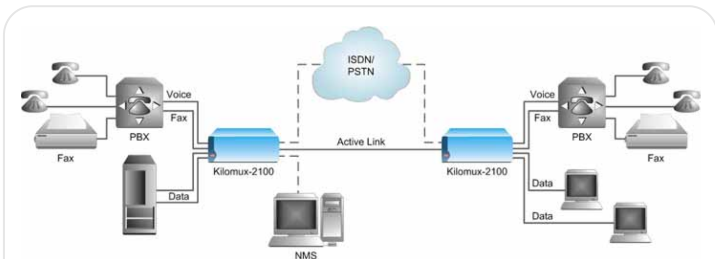
Figure 3. Point-to-point Topology
