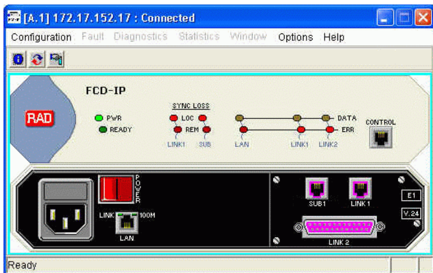
Figure 1. Zoom Application
