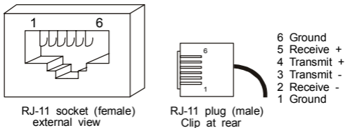
Figure 2. RJ-11 Pin Assignment
