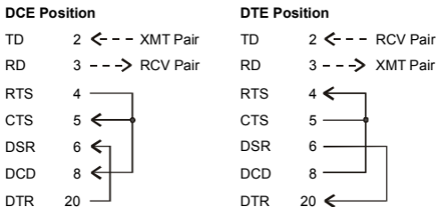
Figure 1. DCE/DTE Switch Configuration
