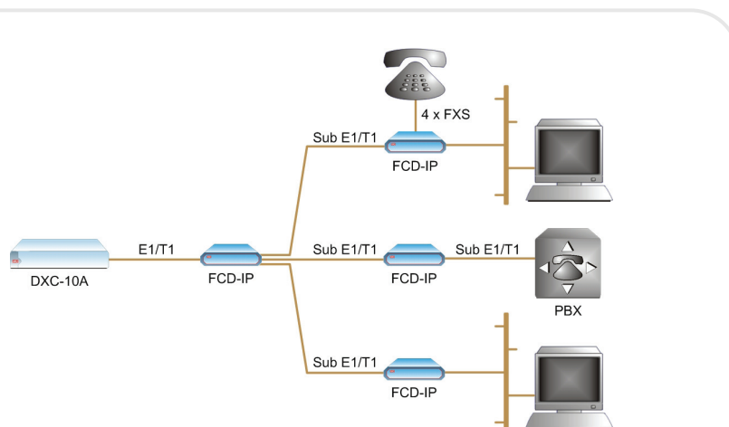
Figure 2. Aggregating Three Fractional E1 Links into One Full E1 Link
