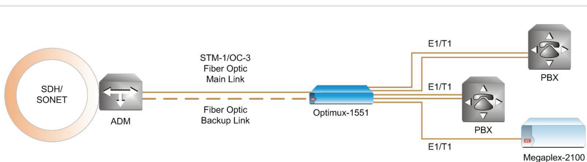
Figure 2. Extending SDH/SONET Service to Remote Customers
